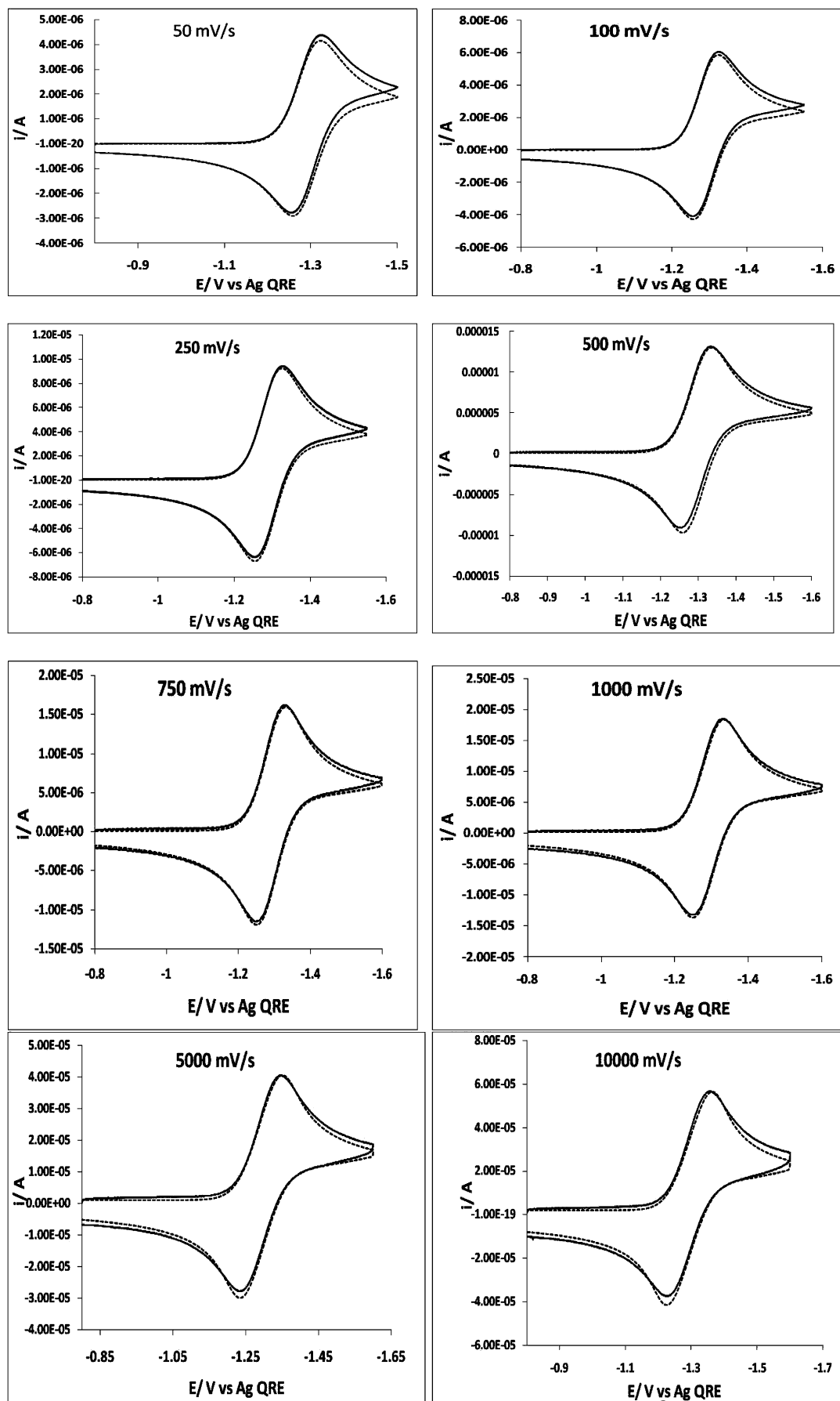
Figure 3. Simulation of reduction of 1 mM BH3. The simulation is corrected for resistance and capacitance: experimental (solid line), simulation (dotted line). The reduction is a one-electron transfer process ( k = 1 \times 10^4 cm/s). R_u = 1.2 k \Omega , C_d = 10 nF, \alpha = 0.5 , D = 9 \times 10^{-6} cm 2 /s.
